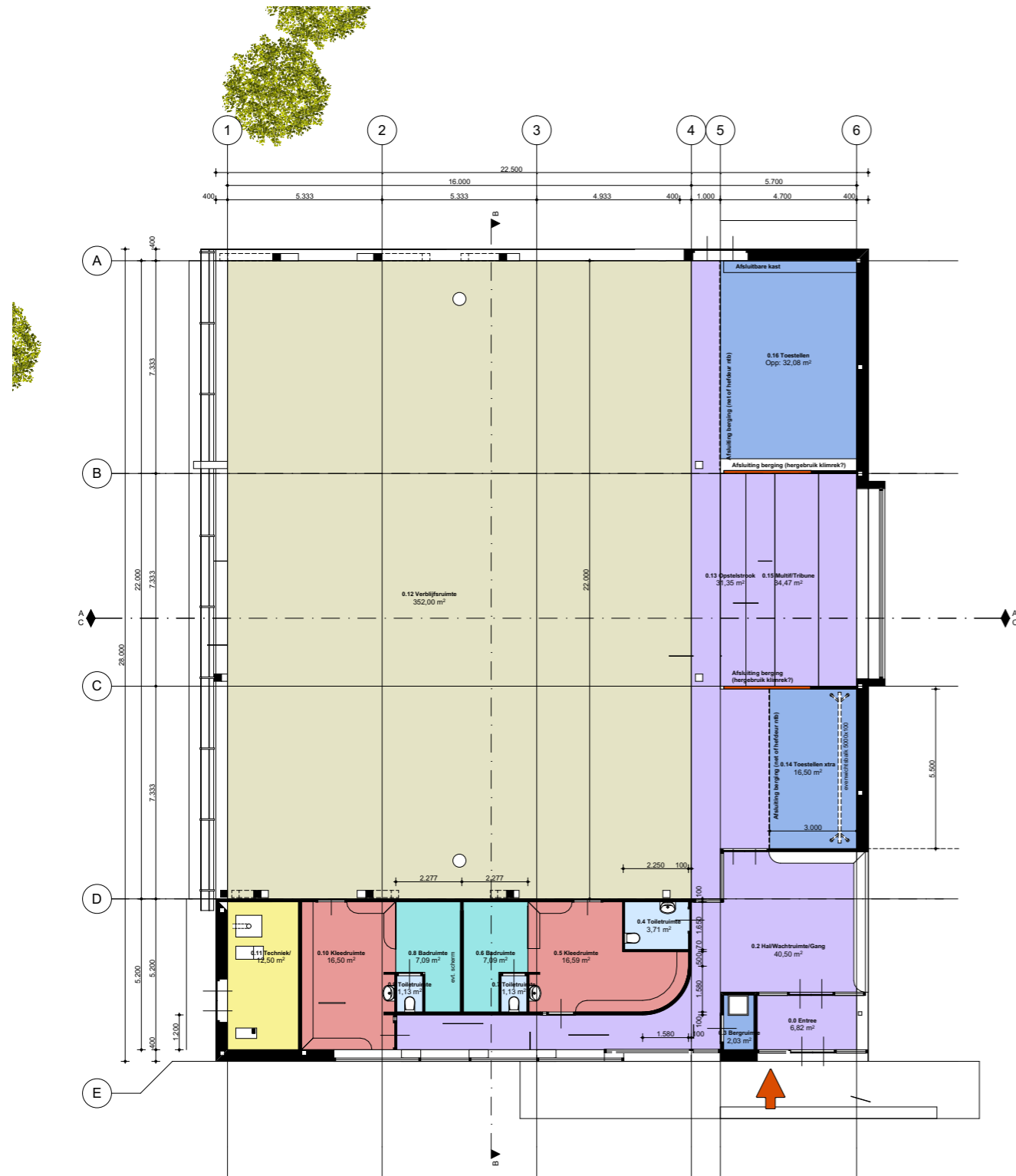
0. Begane grond 1:200
